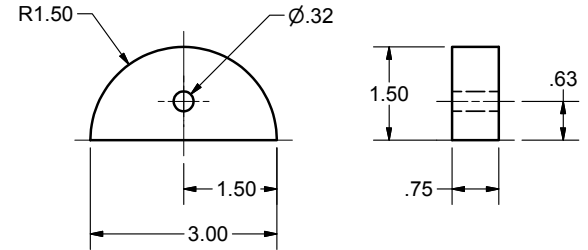
10. ROUND 1 NOTES: 1. TWO REQUIRED 2. SCALE 1:2
